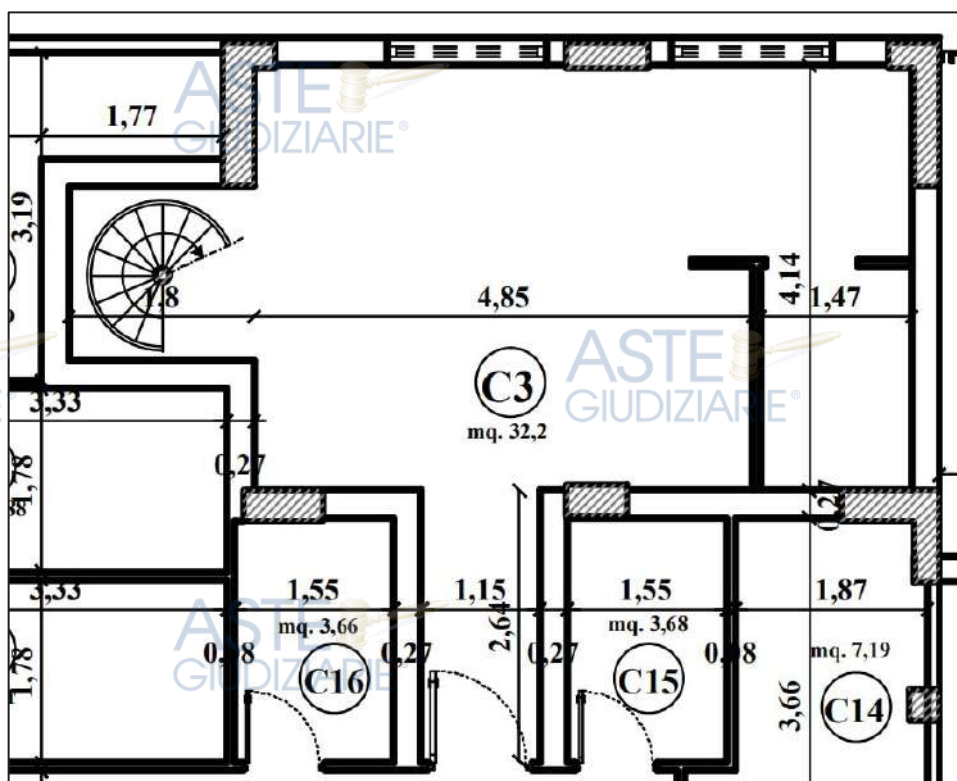
Piano S1
