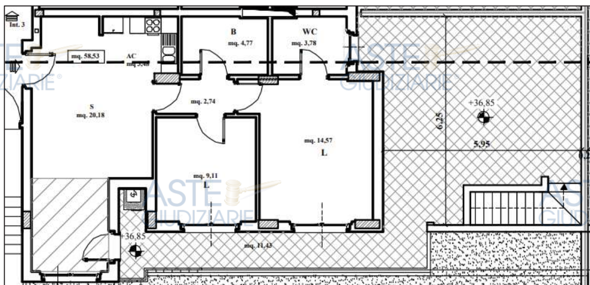
Piano terra
