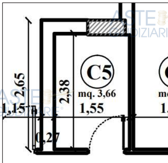
Piano S1
