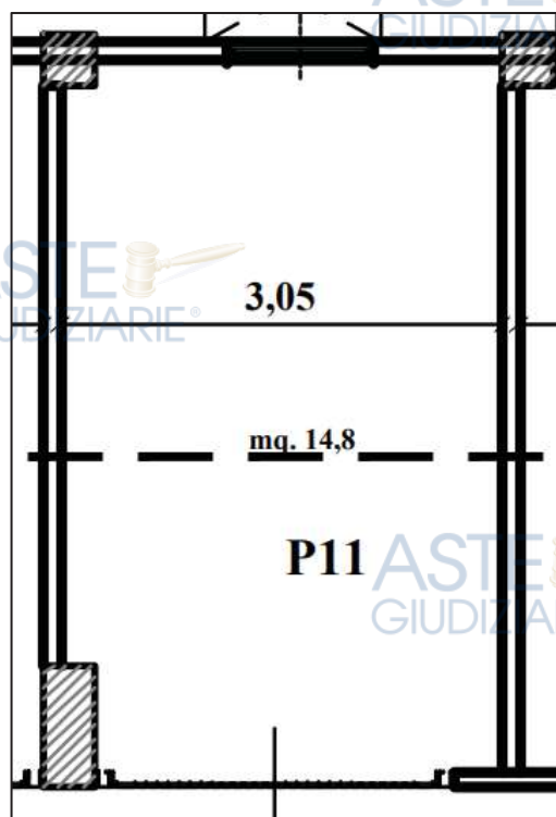
Piano S1
