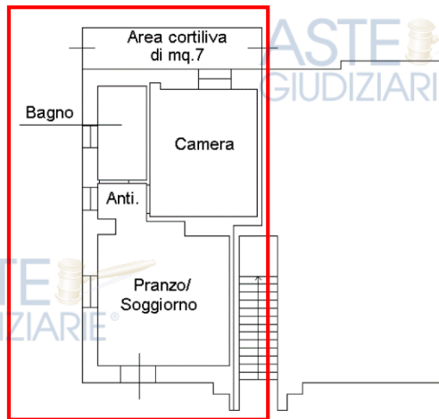
PIANO TERRA(H=230Cm)
