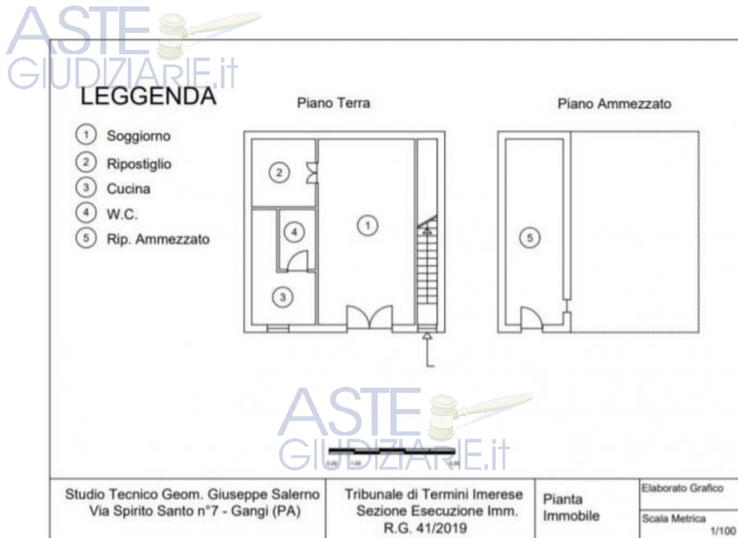
Planimetria Piano T-Amm
