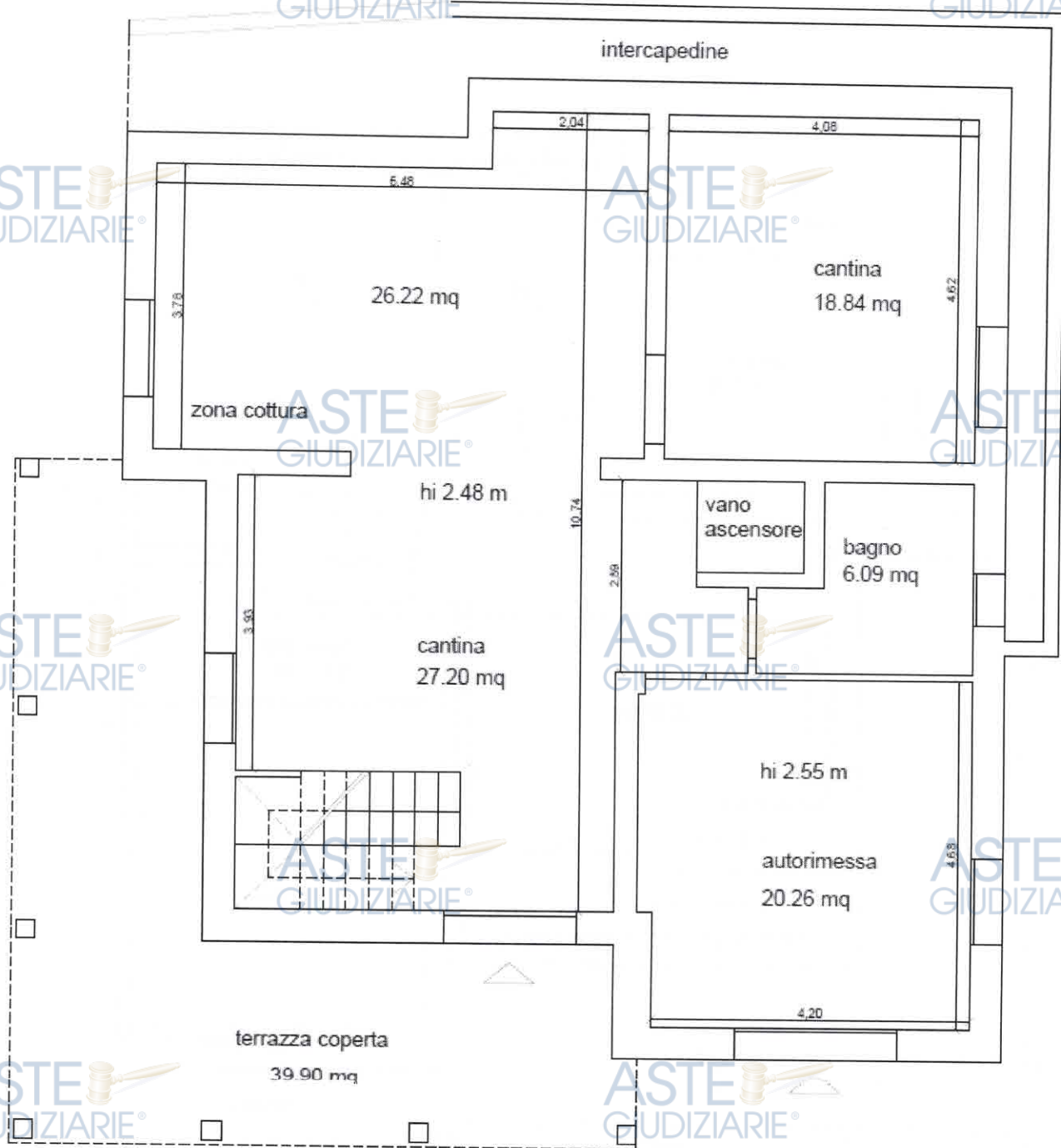
PIANO SEMINTERRATO
