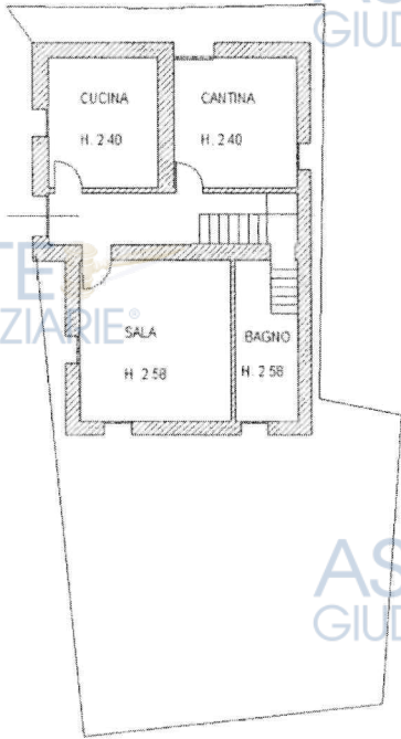
PIANO TERRA
