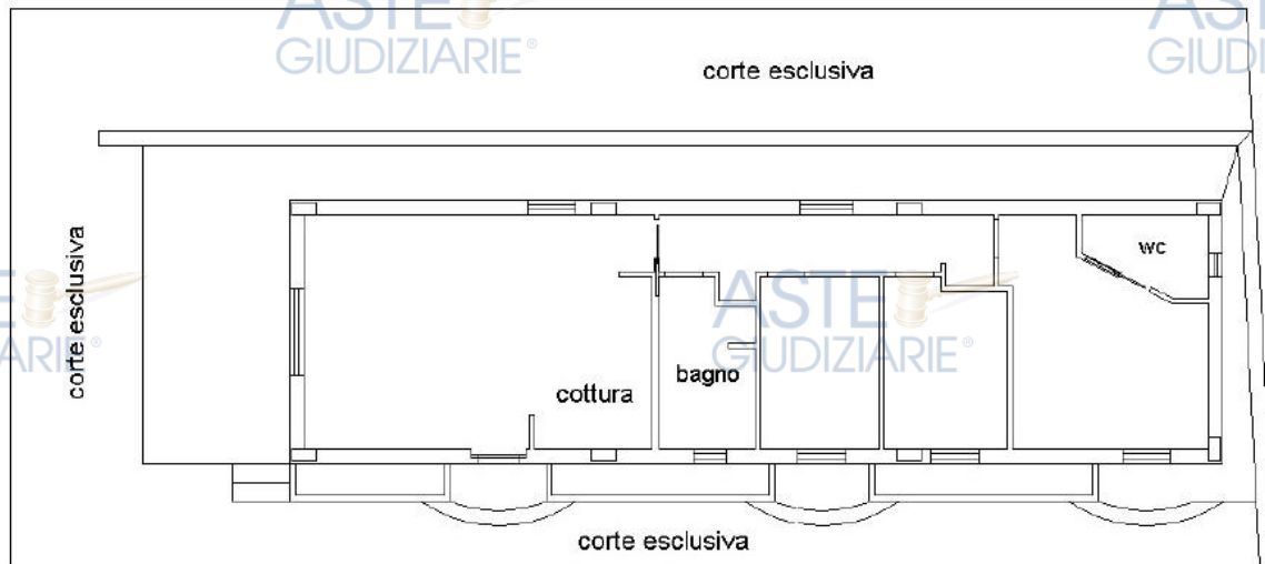
PIANO TERRA hmed=283
