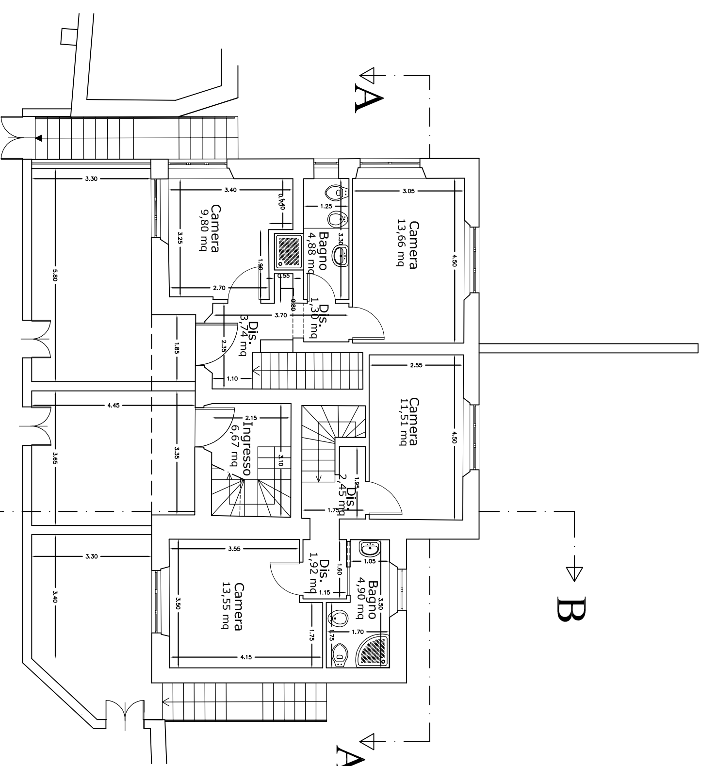
PIANO TERRA
